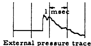
Fig. 26. Typical reflected pressure and external pressure traces.
